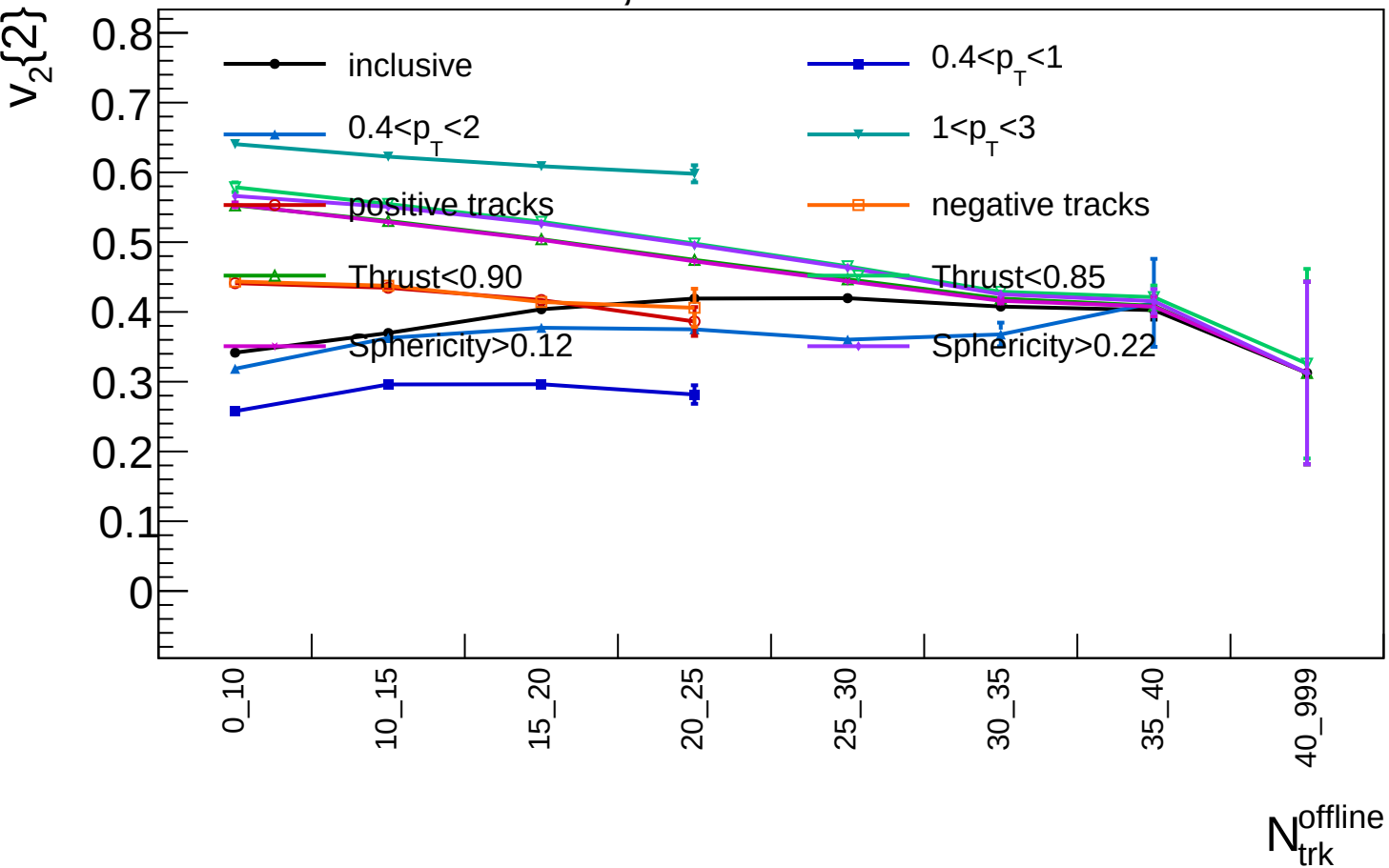
LEP1 reconstructed MC, thrust axis
