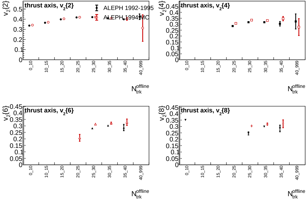
Figure 10: Thrust-axis comparison of LEP1 1992–1995 data and 1994 reconstructed MC. Missing high-order points correspond to sign-invalid cumulants or bins without a valid real-valued v_2\{m\} .
