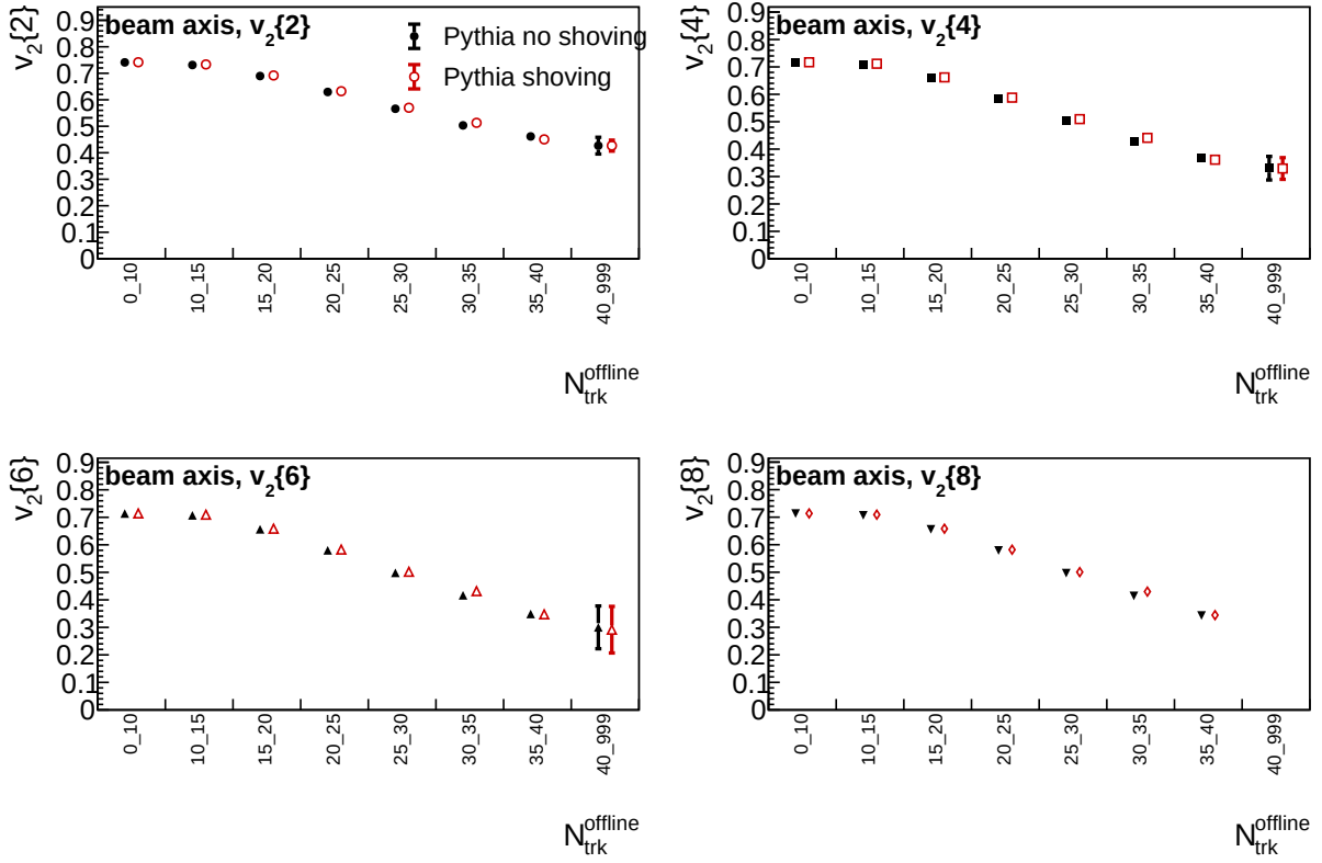
Figure 13: Generator-level Pythia comparison of beam-axis v_2\{m\} with and without Gleipnir shoving. Both samples contain three million accepted hadronic Z-pole events and are processed with the same charged-particle selection and jackknife chunking.
