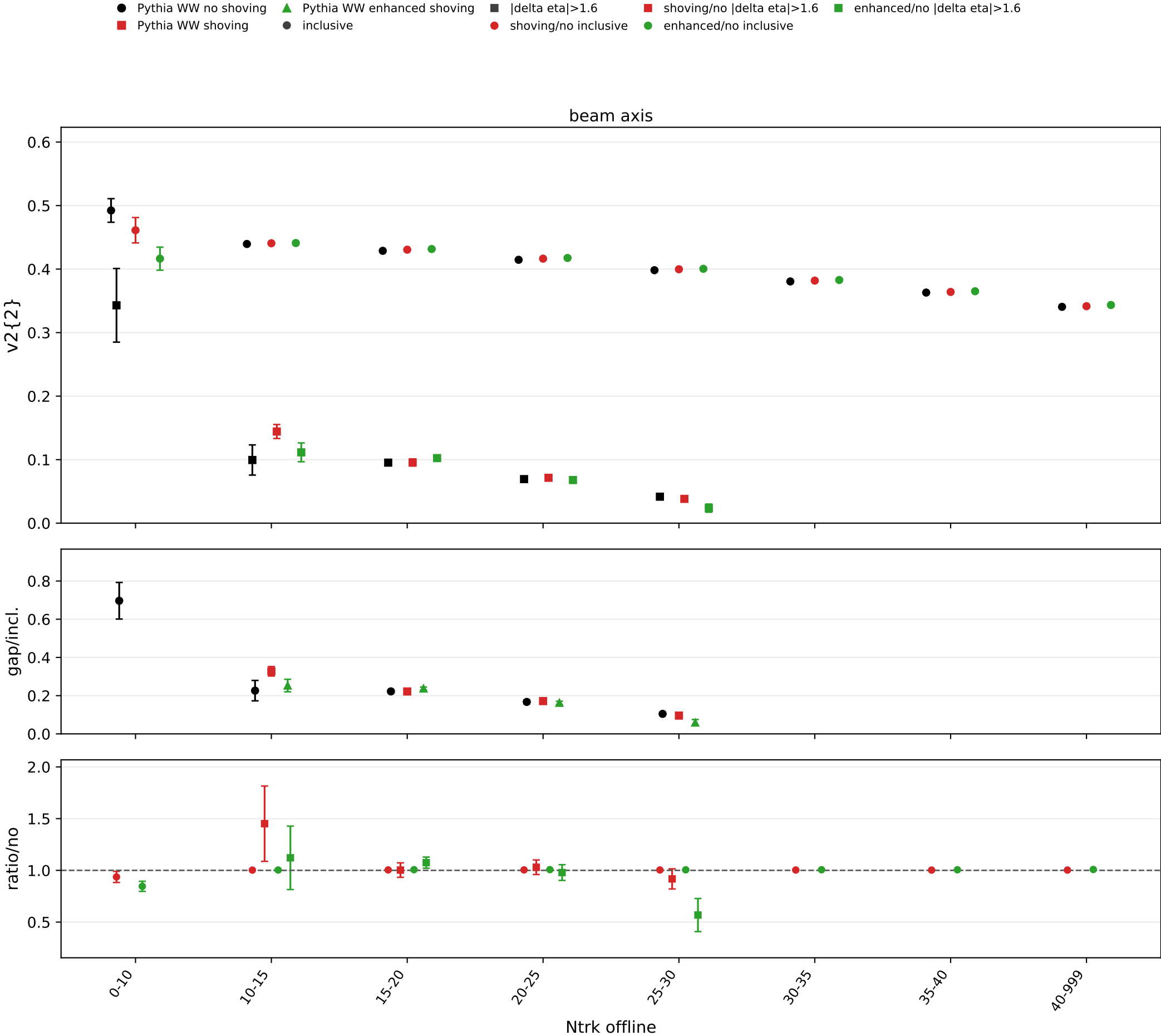
Pythia hadronic WW at 200 GeV, 5M eta-gap comparison, |\Delta\eta| > 1.6
