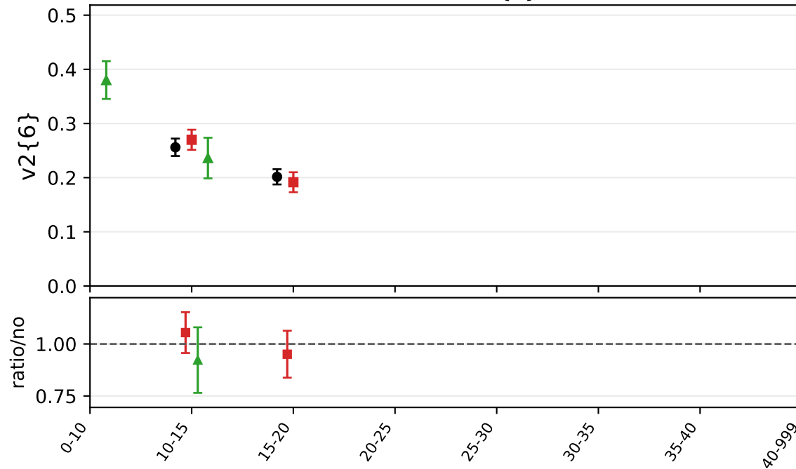
beam axis, v2{6}
