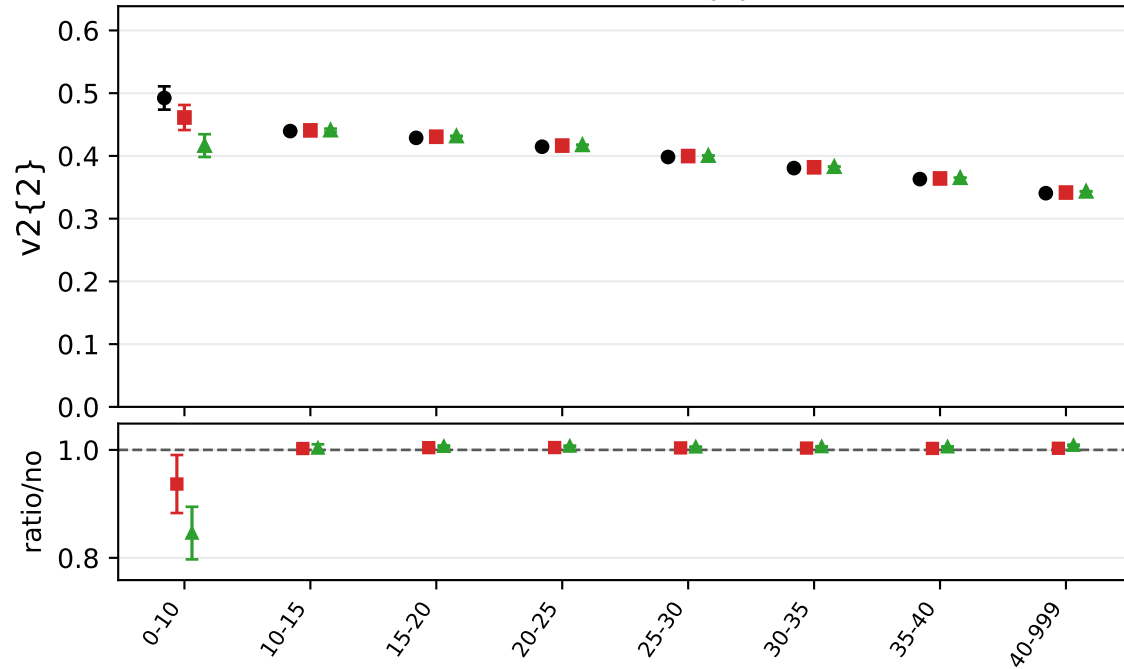
beam axis, v2{2}
