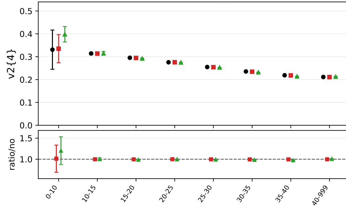
beam axis, v2{4}
