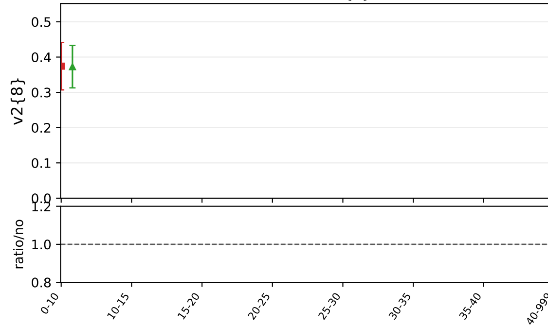
beam axis, v2{8}
