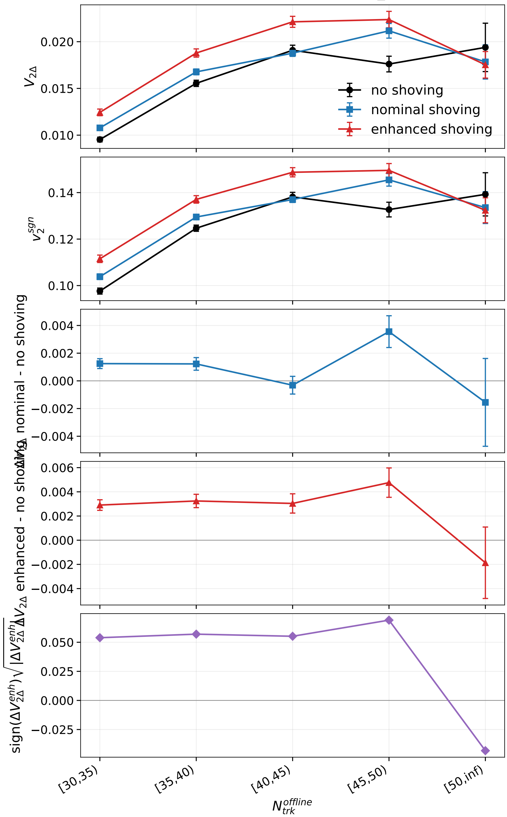
WW 200 GeV long-range thrust-axis V2Delta, high_multiplicity bins
