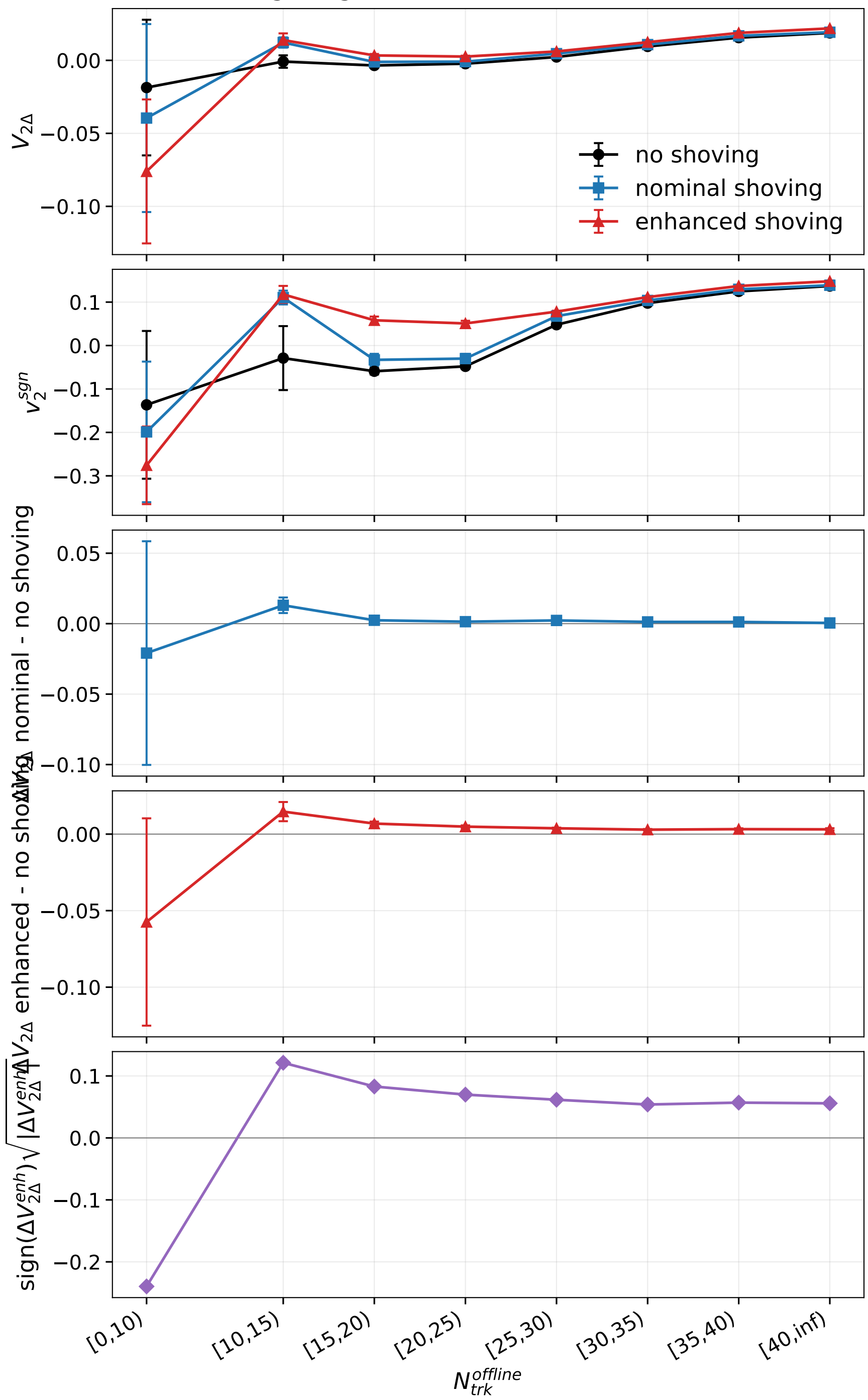
WW 200 GeV long-range thrust-axis V2Delta, standard bins
