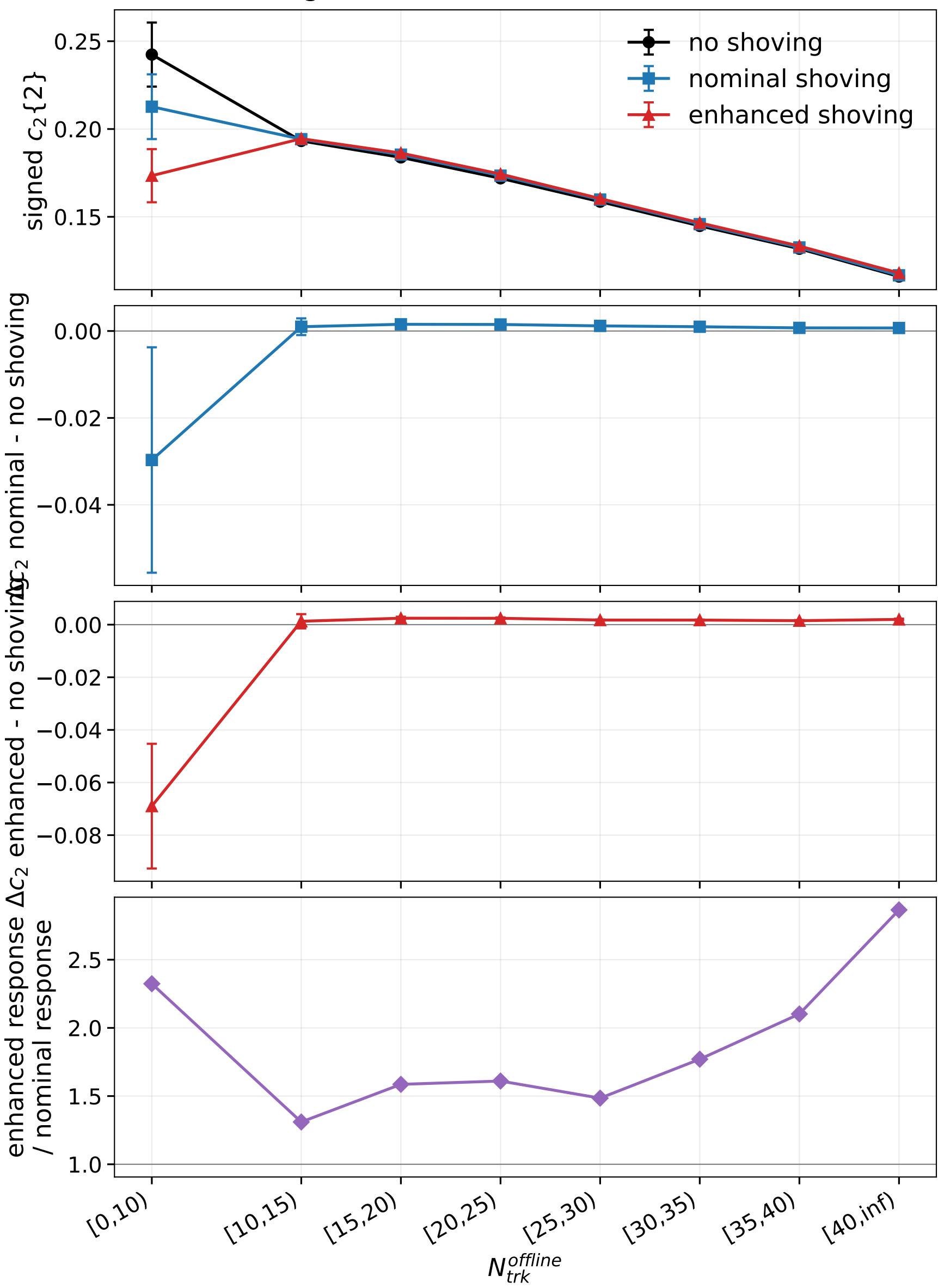
WW 200 GeV signed c2, beam axis, inclusive: inclusive
