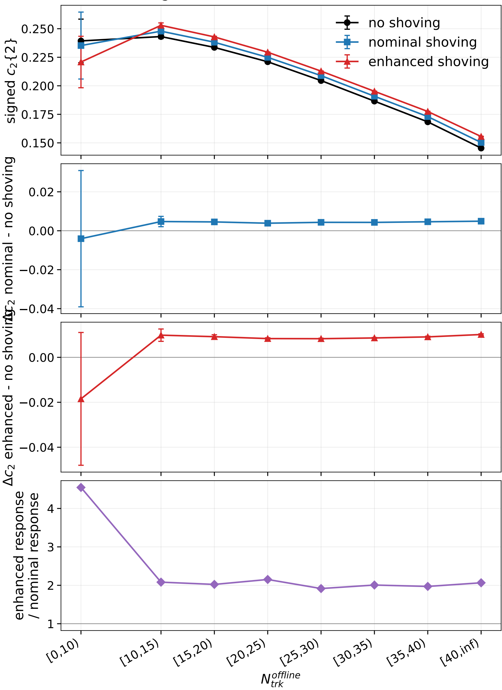
WW 200 GeV signed c2, thrust axis, inclusive: inclusive
