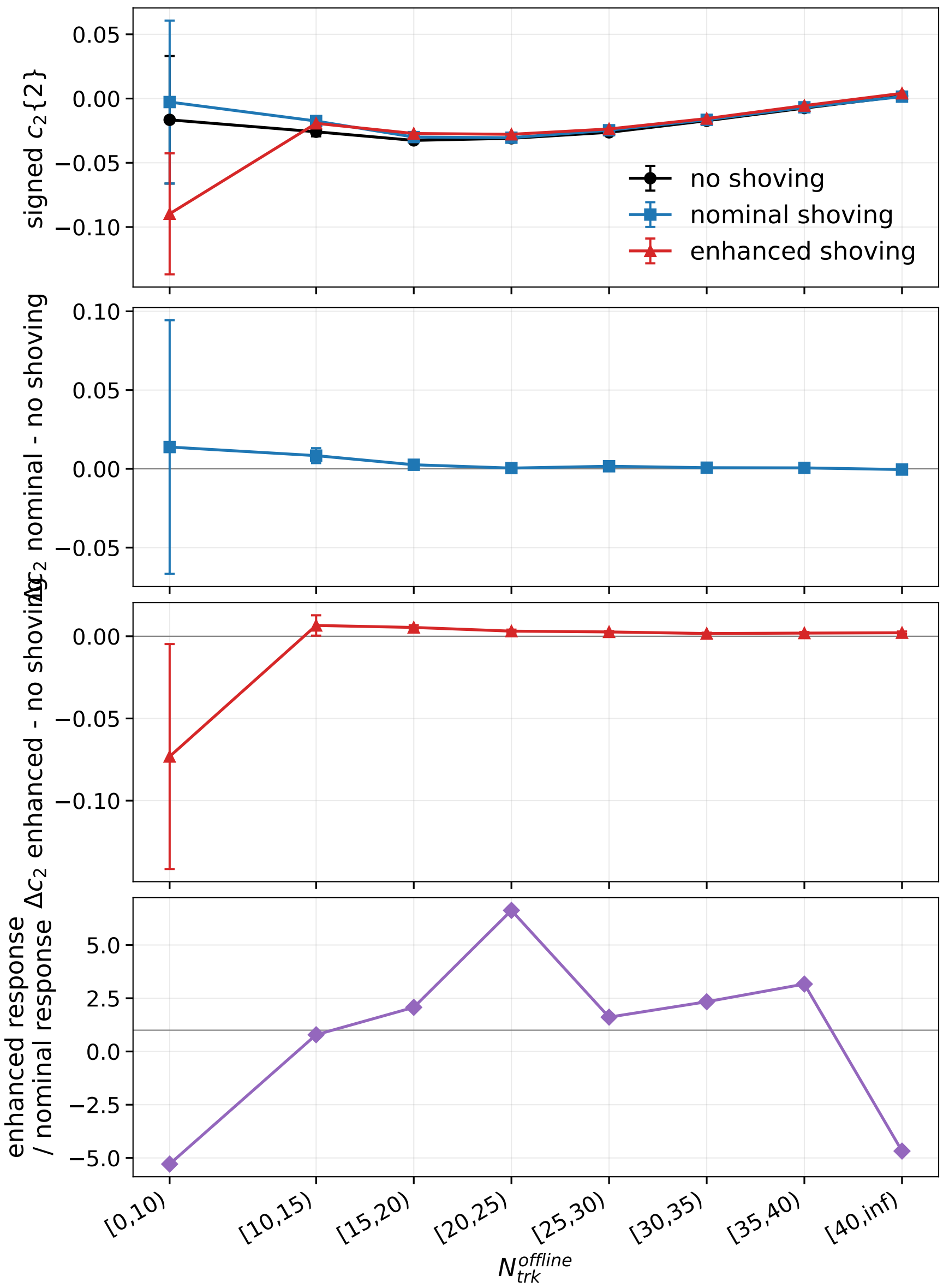
GeV signed c2, thrust axis, two_subevent: eta_lt_minus_0p5_vs_eta
