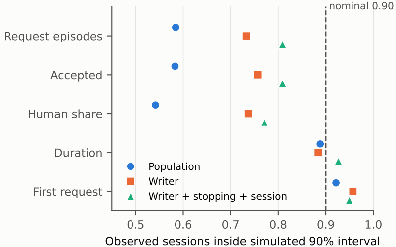
(b) Later sessions of known writers
