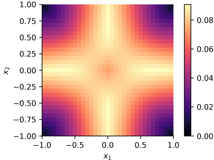
Critic 32 2 : nodal error
