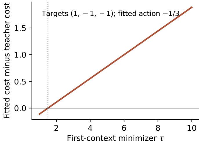
Same targets; opposite cost effects
