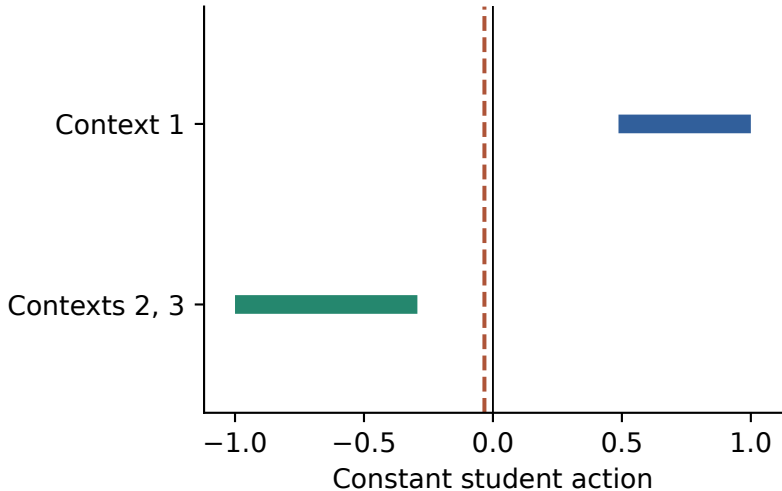
No common feasible fit ( \alpha = 1/2 )
