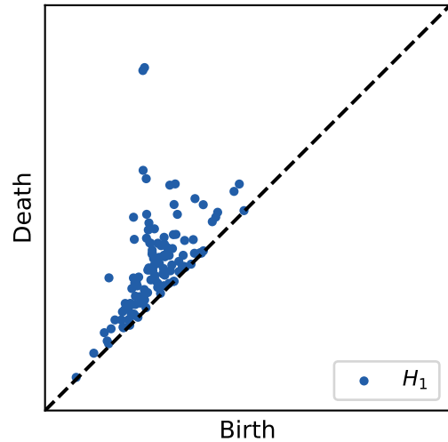
Persistence diagram 2
