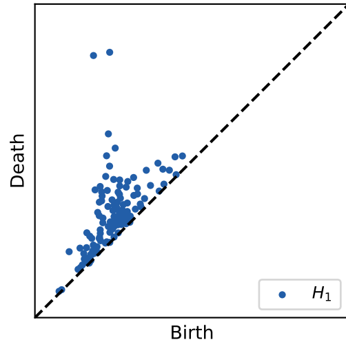
Persistence diagram 3
