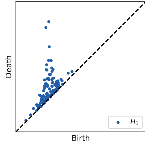
Persistence diagram 1
