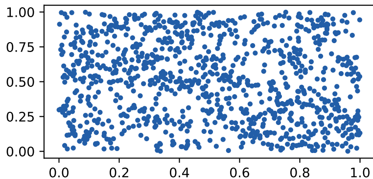
r=2.5 Point cloud
