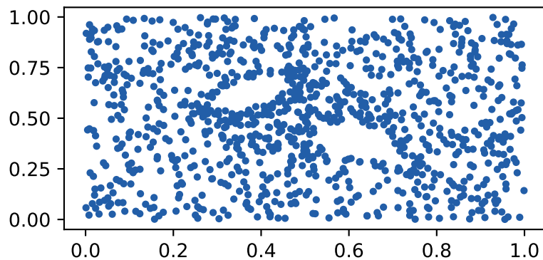
r=4.3 Point cloud
