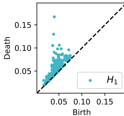
Persistence diagram
