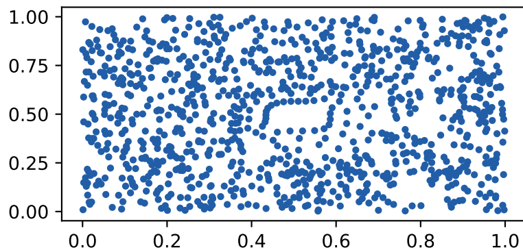
r=4.0 Point cloud
