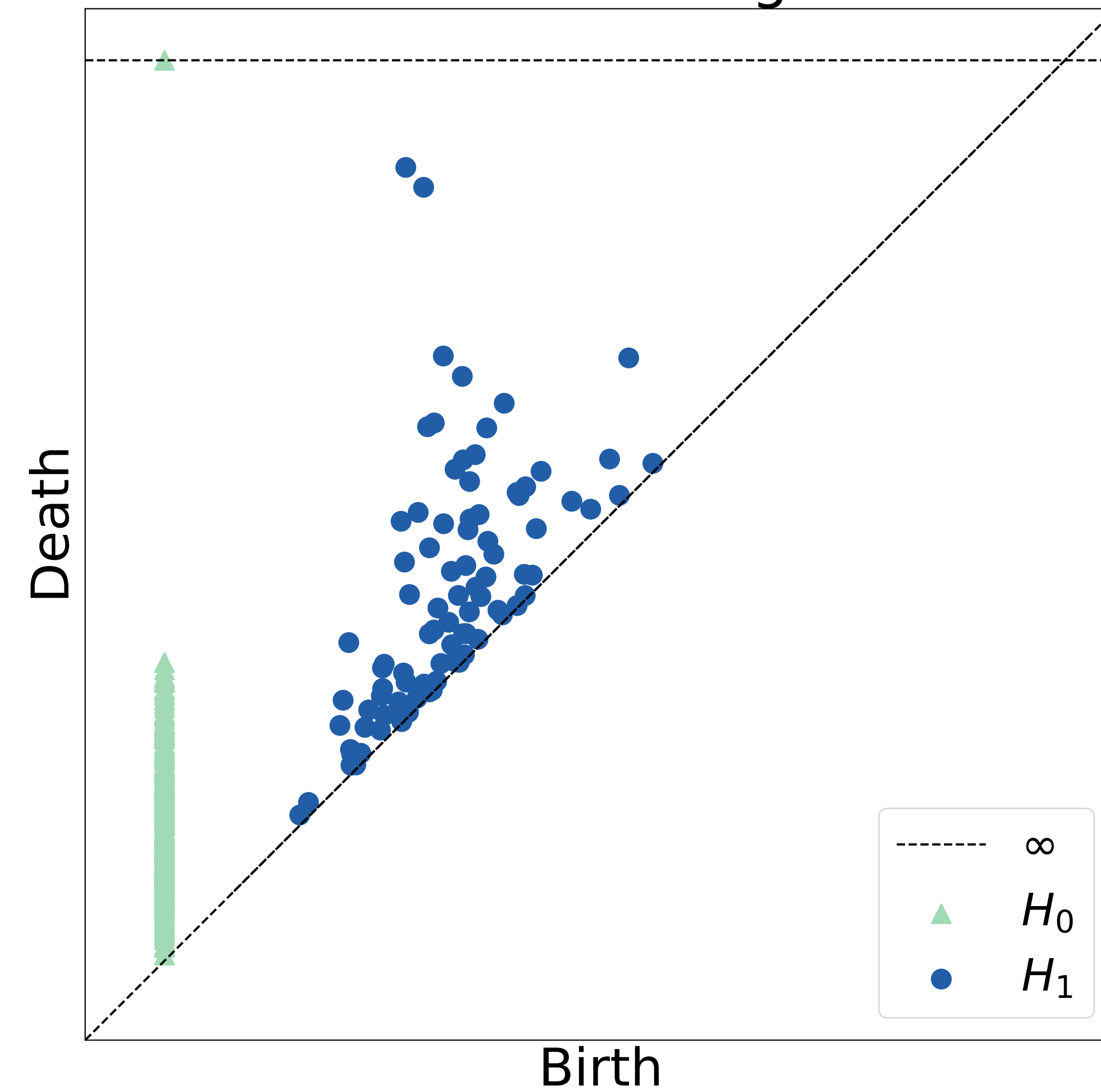
Persistence Diagram
