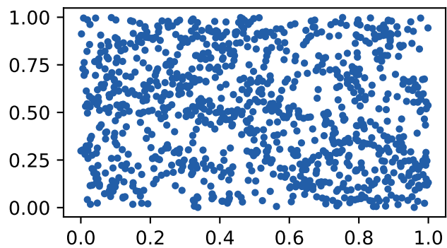
r=2.5 Point cloud
