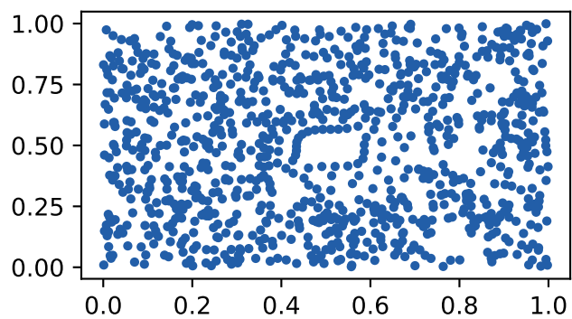
r=4.0 Point cloud
