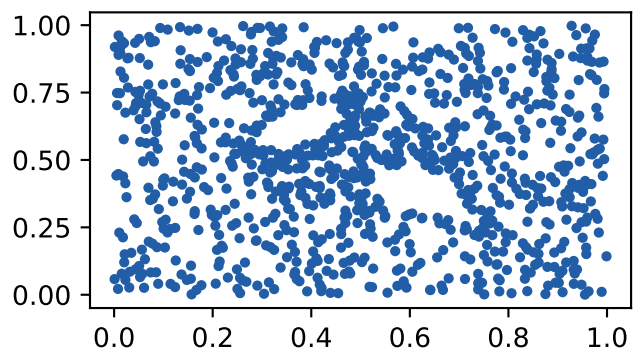
r=4.3 Point cloud
