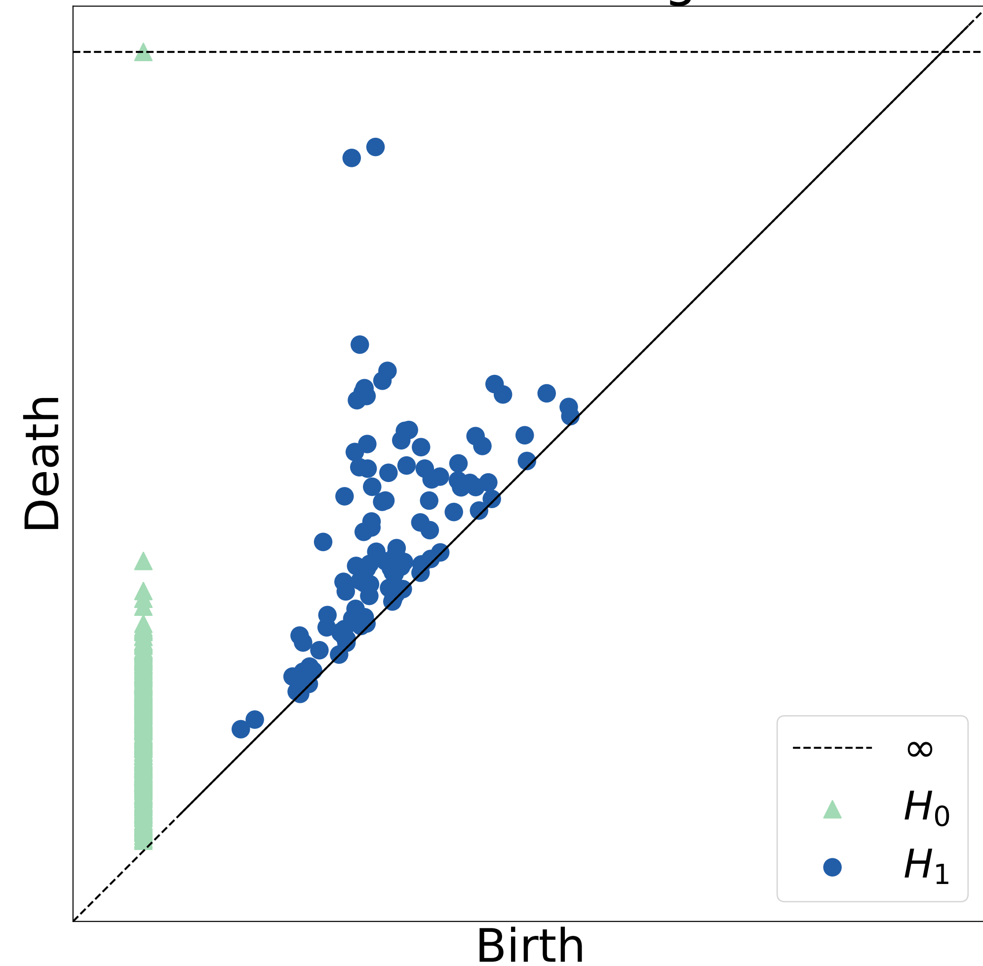
Persistence Diagram
