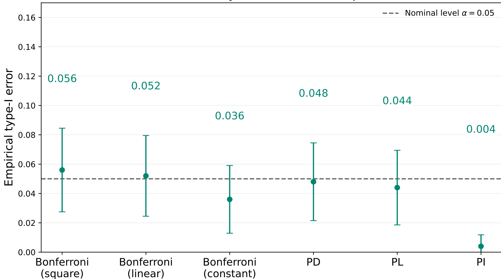
Torus null validity (n=m=50, 250 replications)
