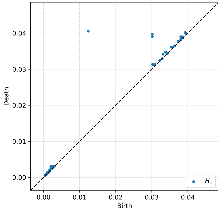
Persistence Diagram of a clarinet
