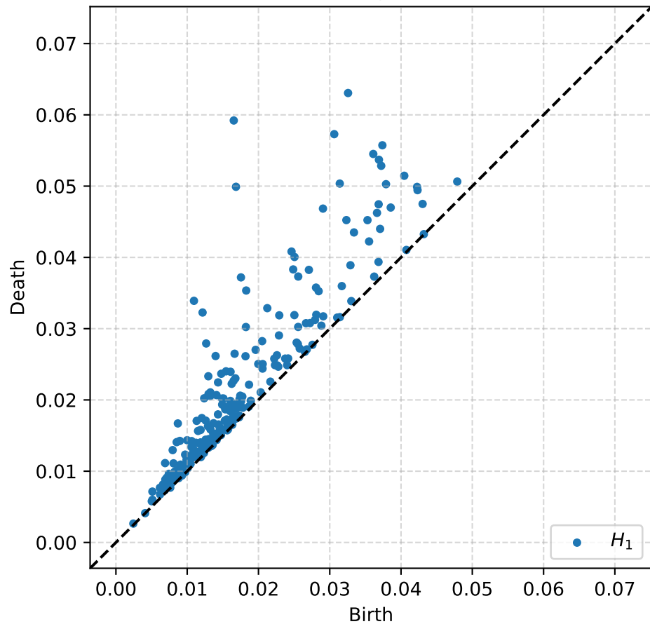
Persistence Diagram of a flute
