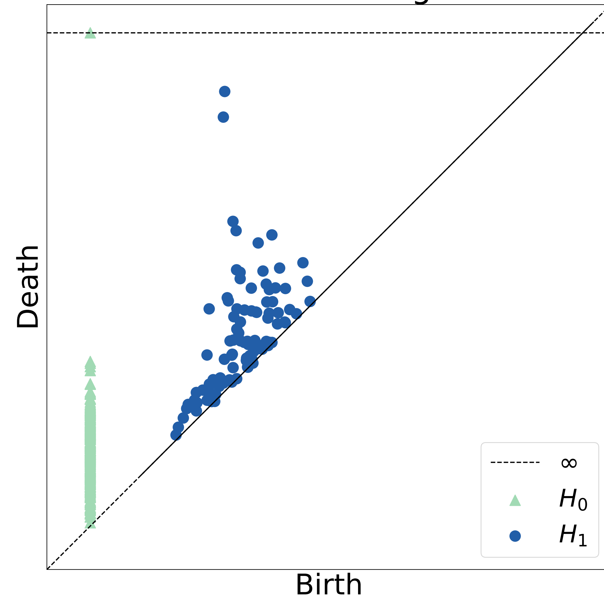
Persistence Diagram
