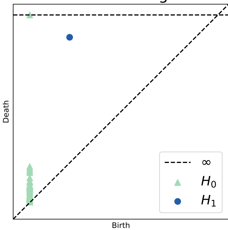
Persistence diagram
