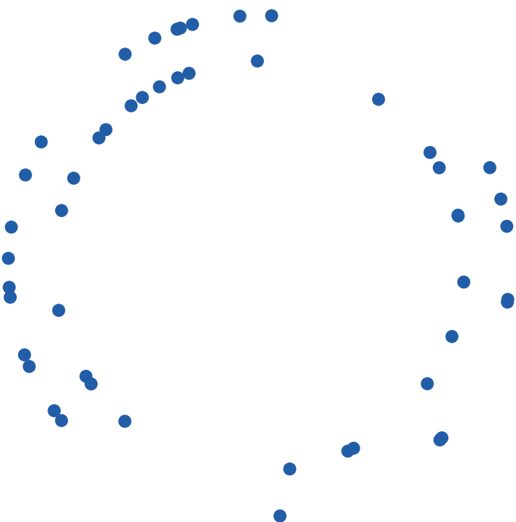
Point cloud on two concentric circles
