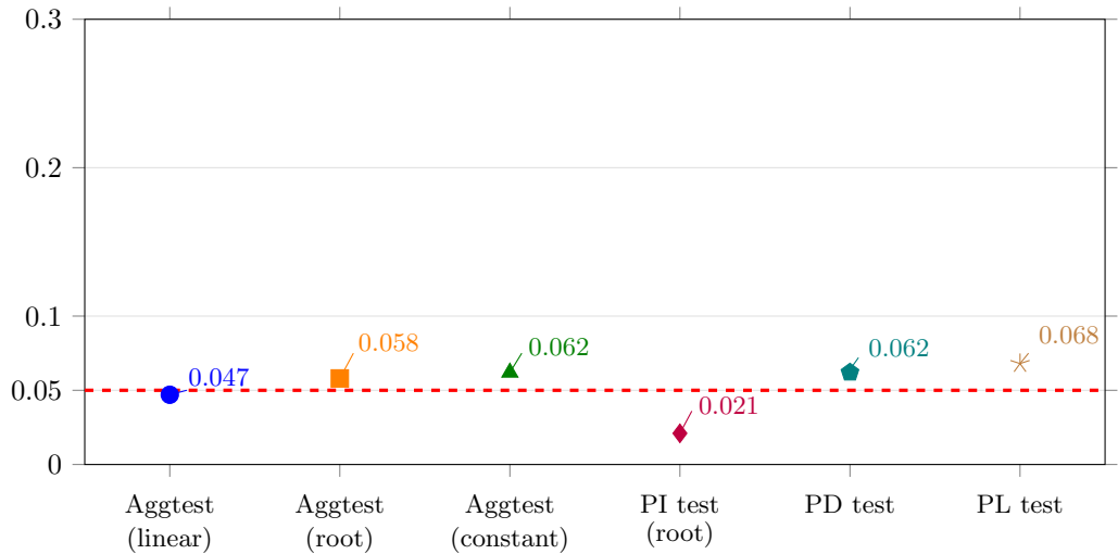
Empirical Type I error
