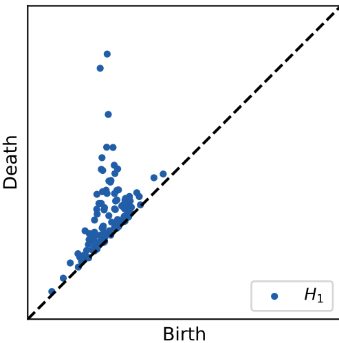
Persistence diagram 1
