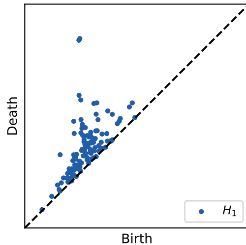
Persistence diagram 2
