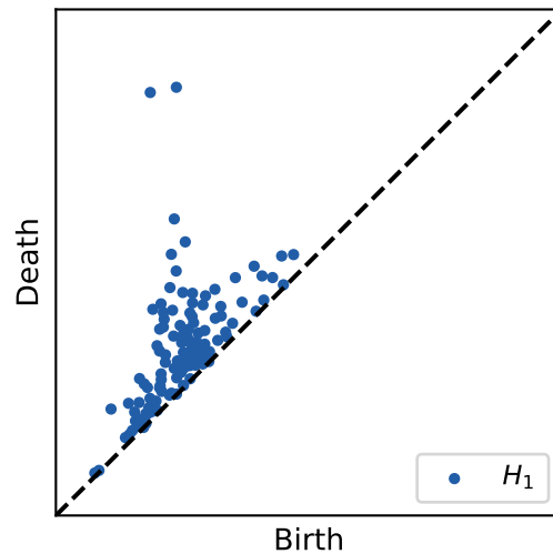
Persistence diagram 3
