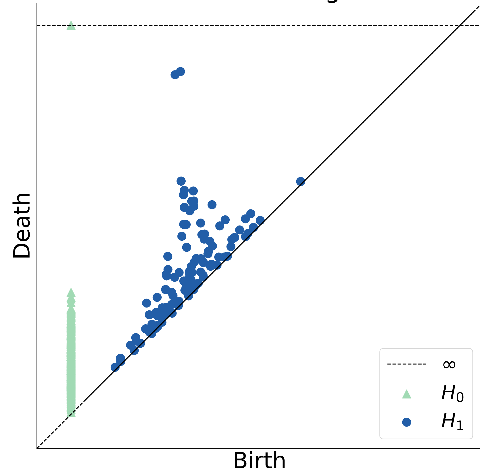
Persistence Diagram
