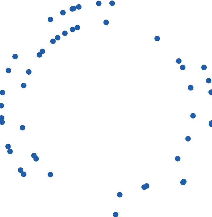
Point cloud on two concentric circle
