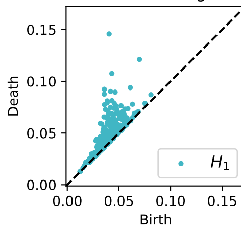
Persistence diagram
