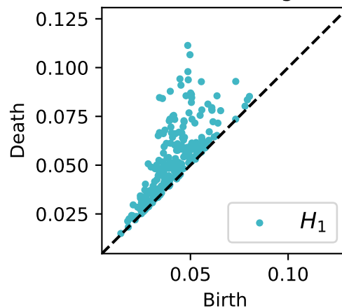
Persistence diagram
