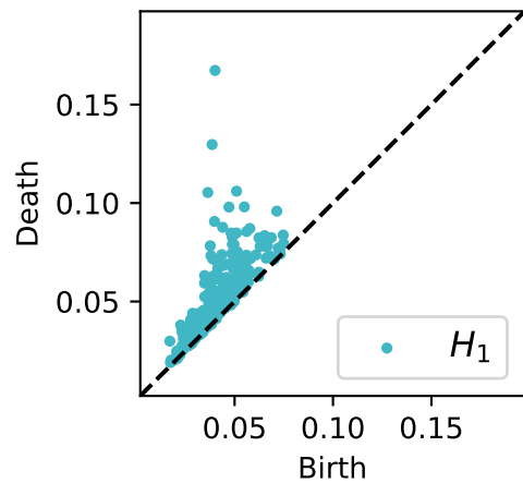
Persistence diagram
