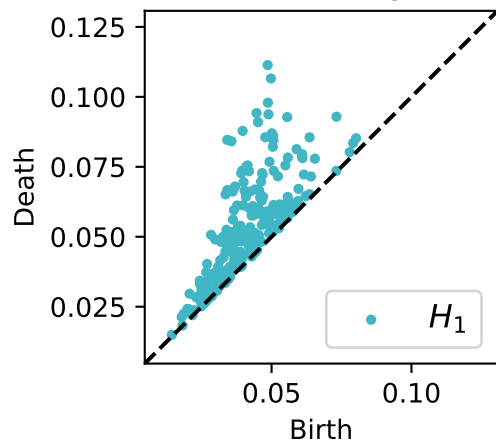
Persistence diagram
