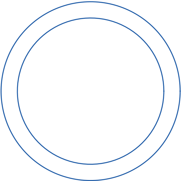
Two concentric circles
