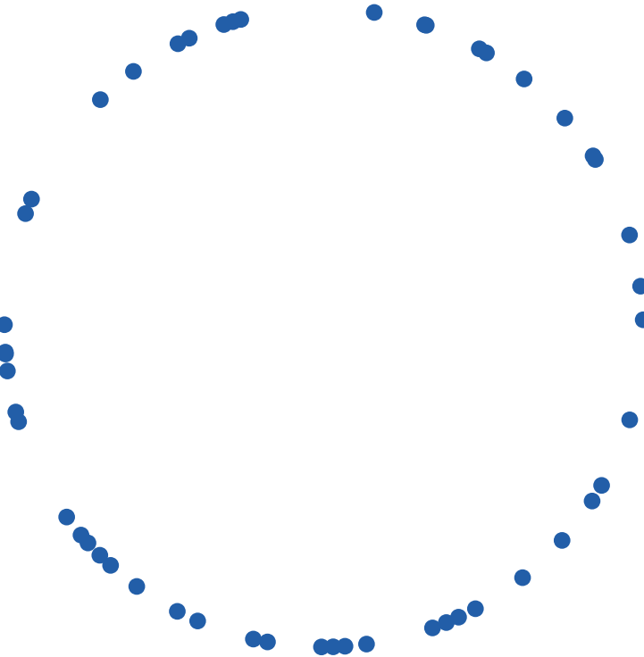
Point cloud on the single circle
