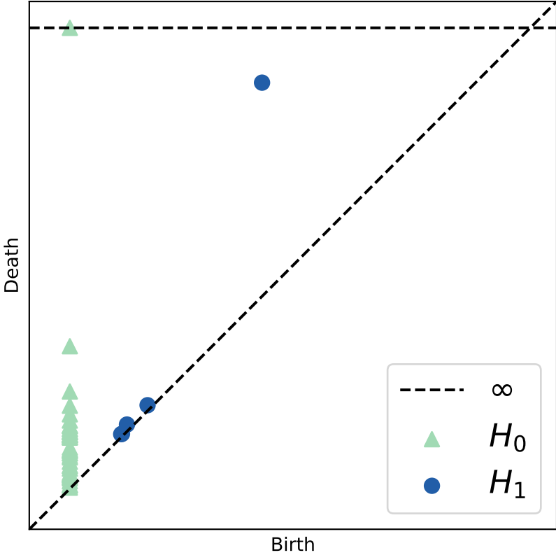
Persistence diagram
