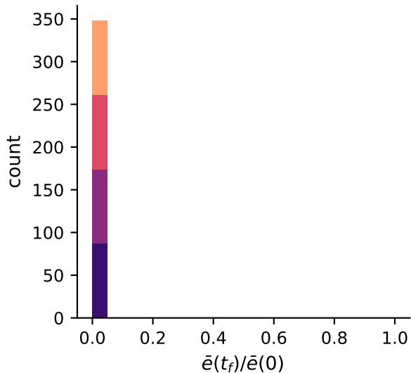
Diverging A^*
