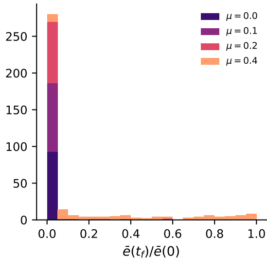
Finite A^*
