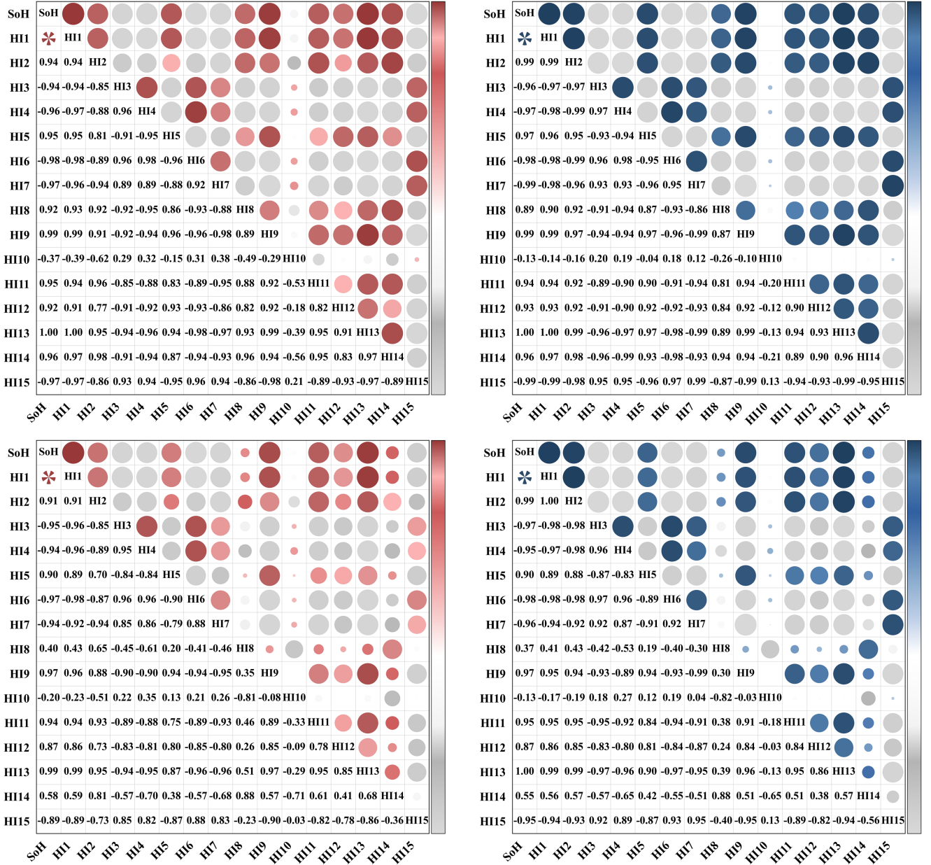
Fig. 4. Correlation matrices of candidate HIs and SOH on the Oxford dataset.
