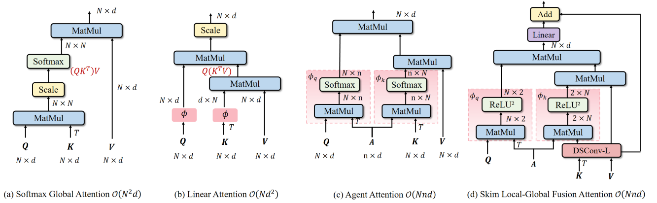
Fig. 7. Comparison of (a) Softmax attention, (b) linear attention, (c) Agent Attention, and (d) the proposed SLFA module.
