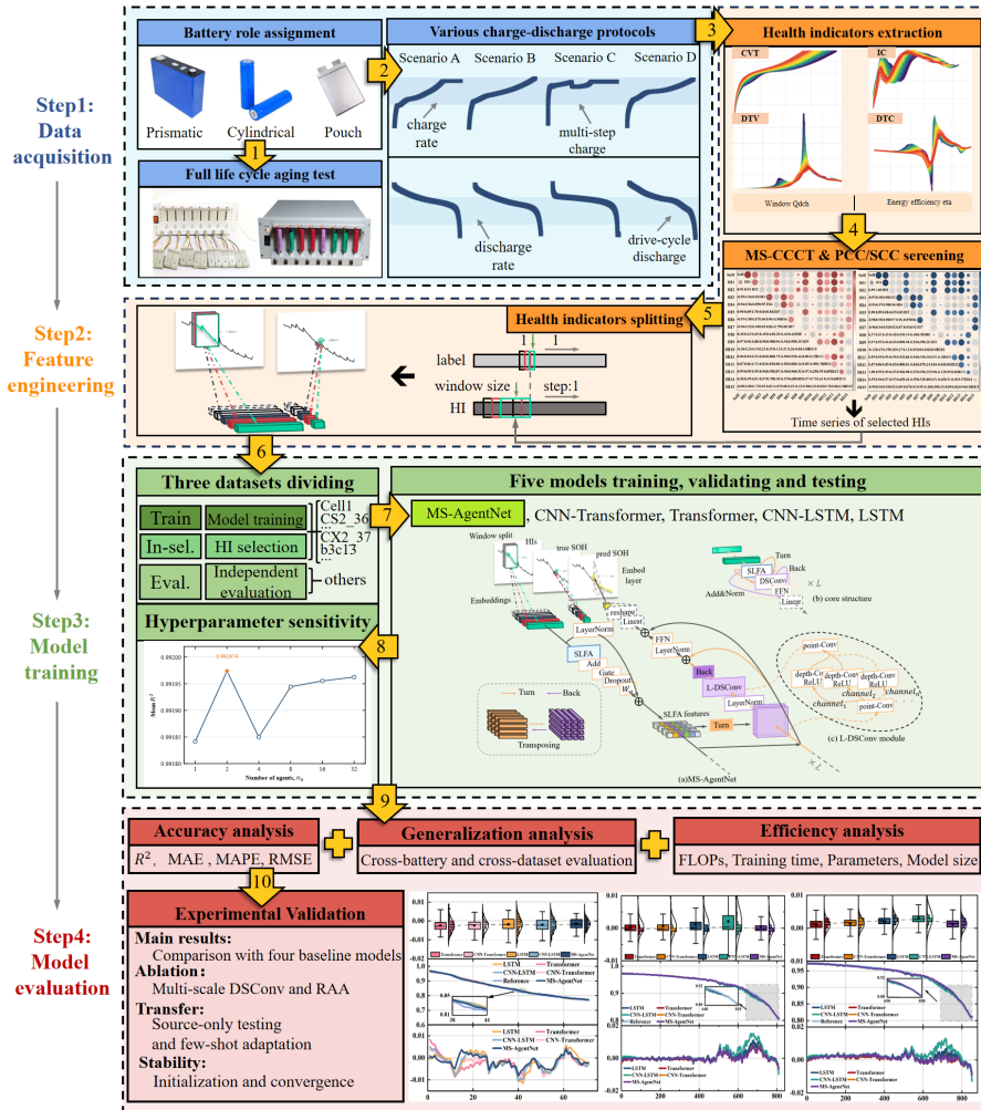
Fig. 1. Flowchart of the developed SOH estimation approach.
