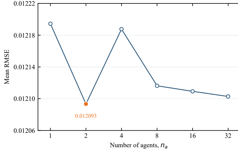
Fig. 8. Mean validation RMSE of MS-AgentNet with different numbers of agents.
