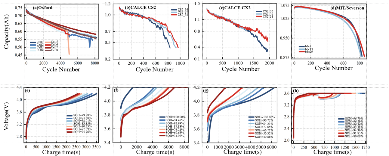
Fig. 2. Four battery datasets: (a)–(d) capacity degradation curves of Oxford, CALCE CS2, CALCE CX2, and MIT/Severson cells, respectively; (e)–(h) charging voltage curves of the four datasets in the same order.
