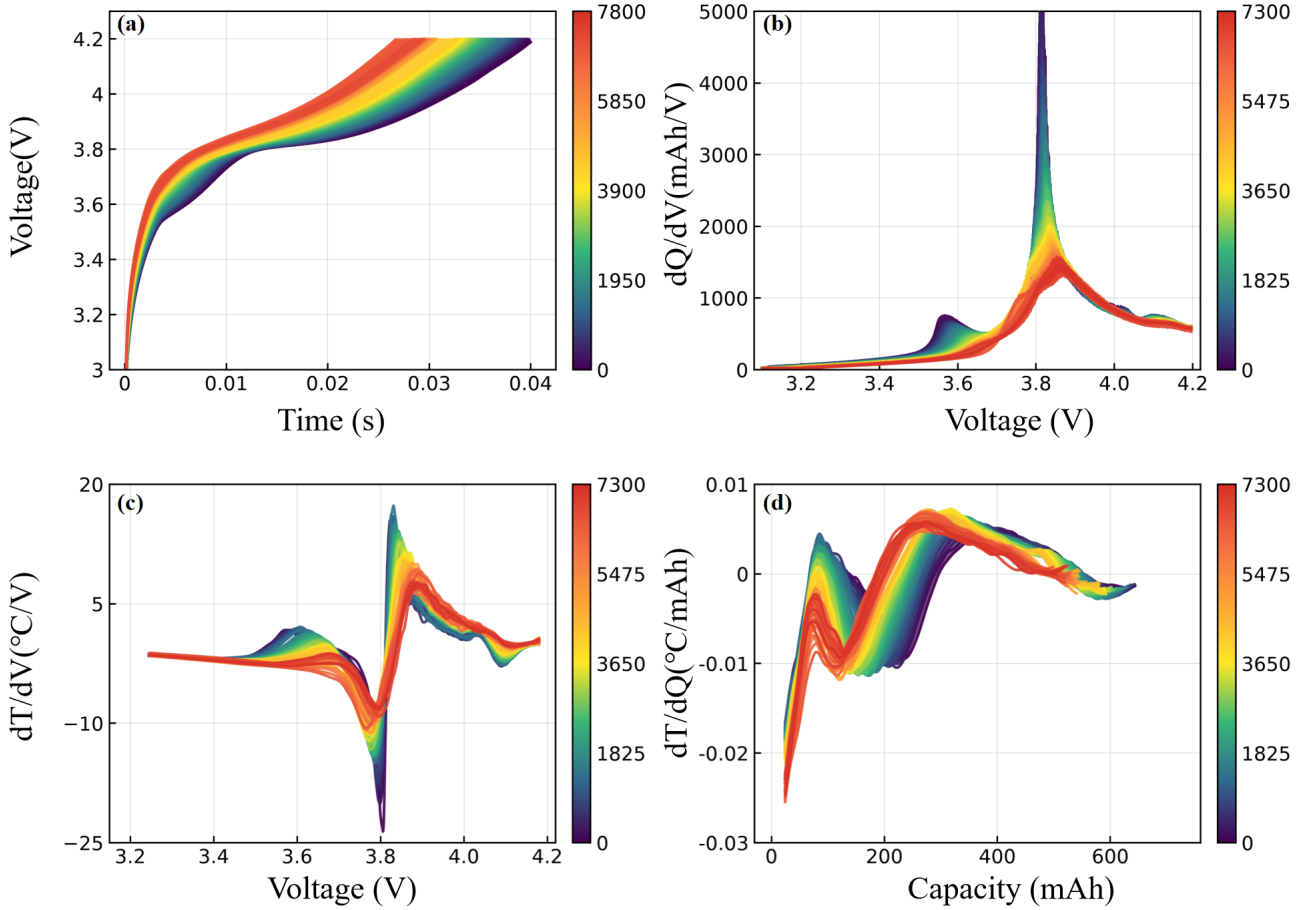
Fig. 3. Charge-side characteristic curves used for HI construction.
