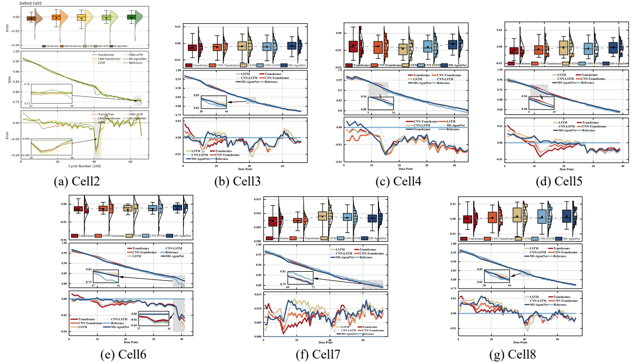
Fig. 8. SOH estimation results of different models on the Oxford dataset.
