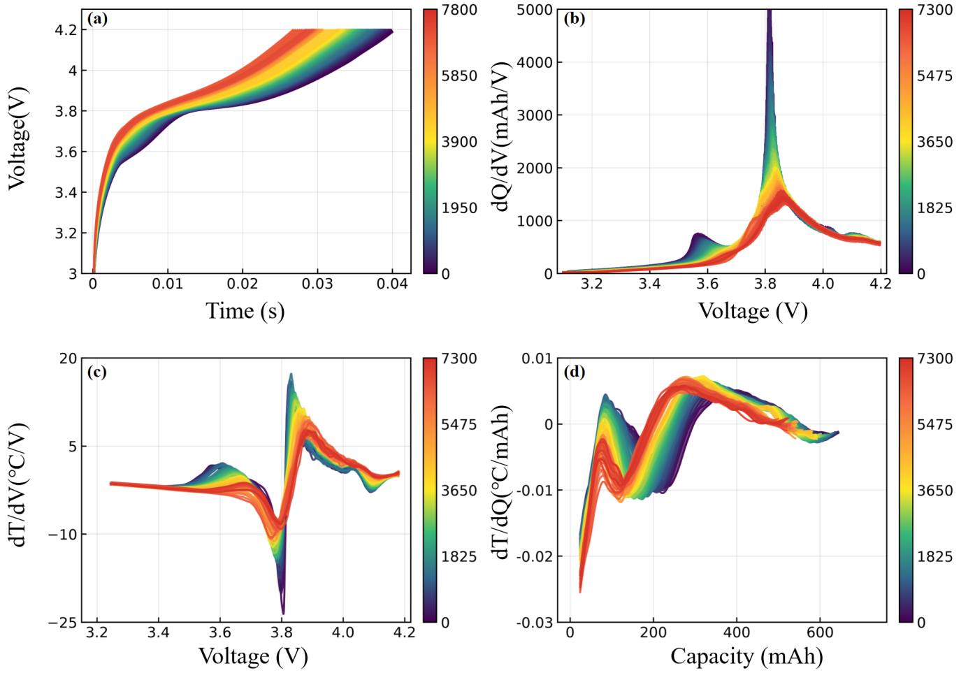
Fig. 3. Charge-side characteristic curves used for HI construction.
