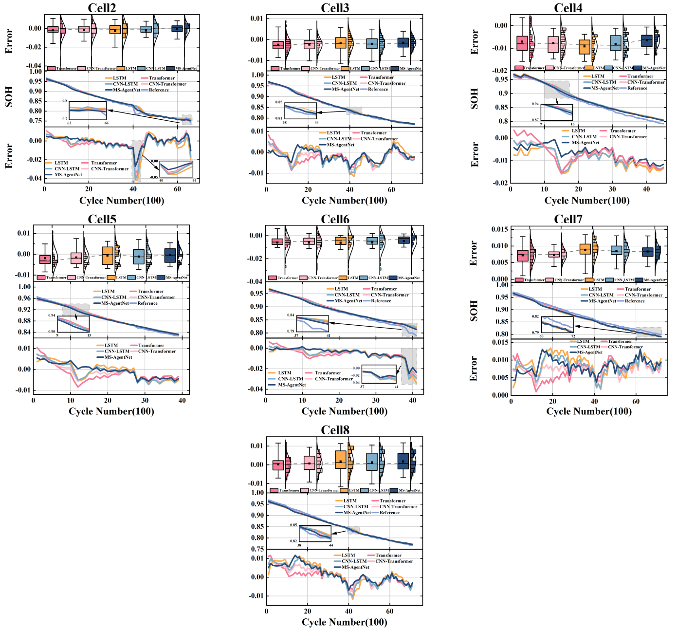
Fig. 8. SOH estimation results of different models on the Oxford dataset.
