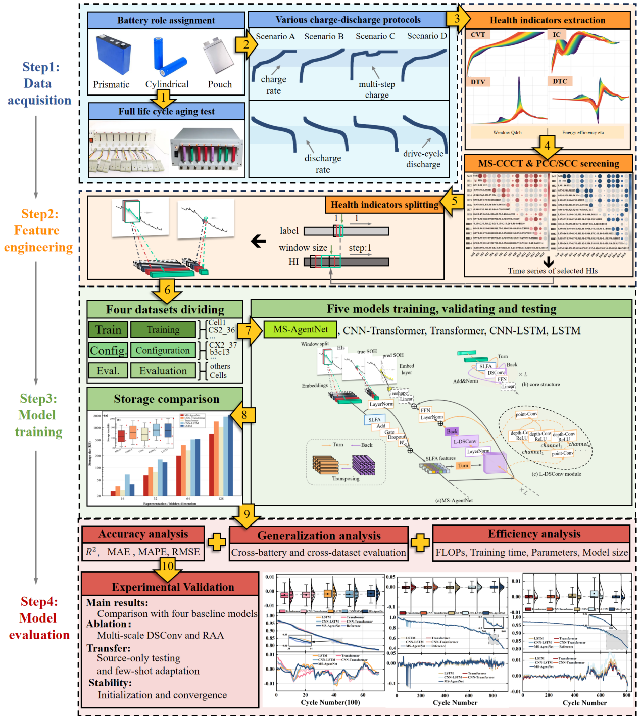
Fig. 1. Flowchart of the developed SOH estimation approach.
