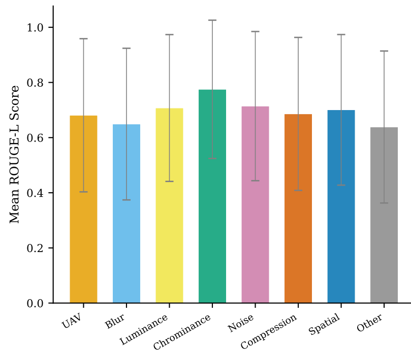
ROUGE-L (Recall)
