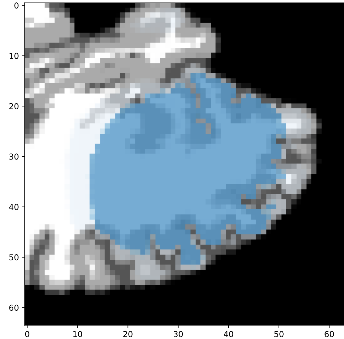
Step 20: Prediction
