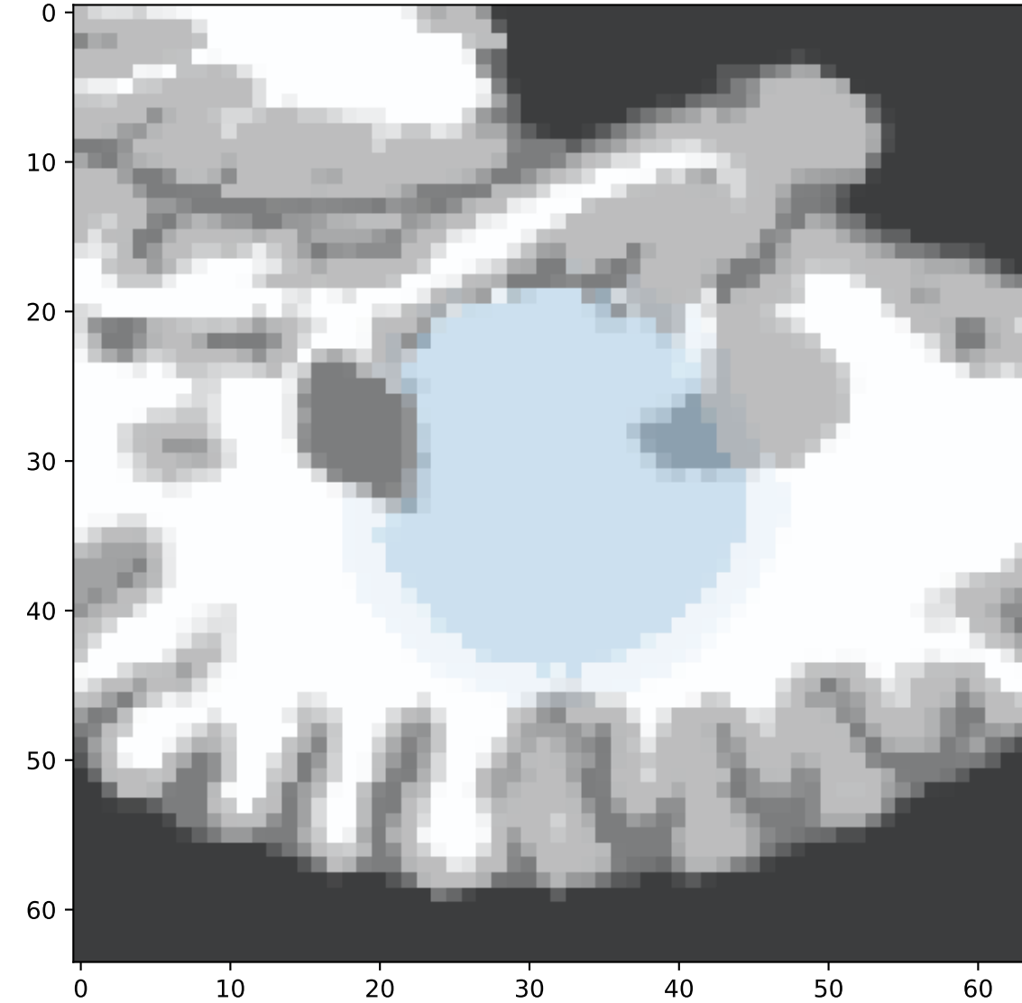
Step 160: Prediction
