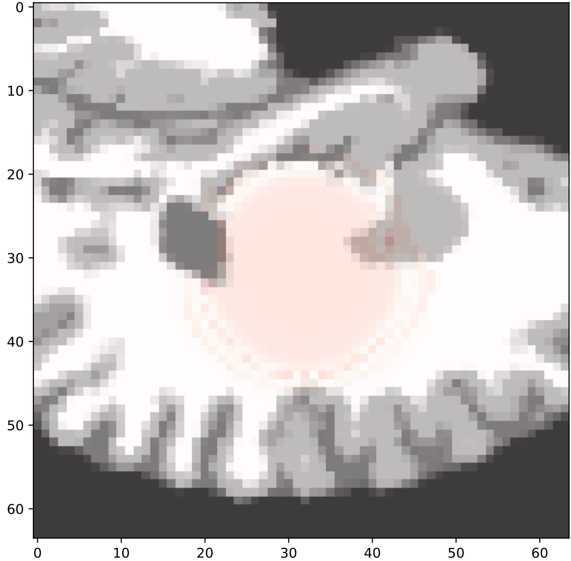
Step 160: Difference
