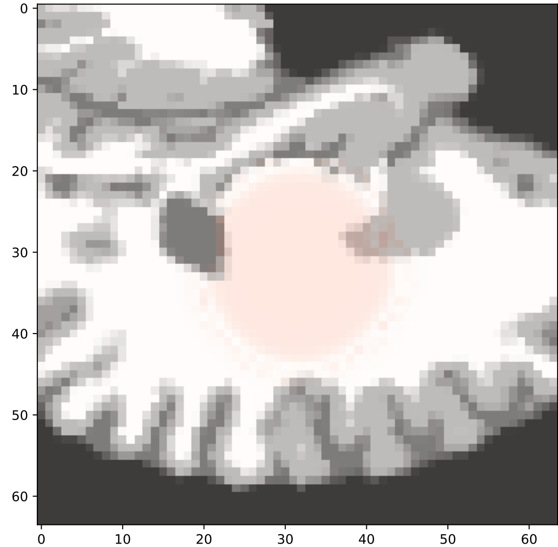
Step 60: Difference
