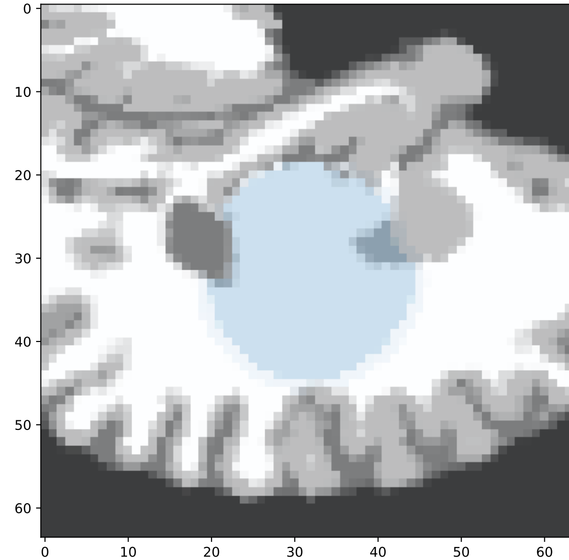
Step 60: Prediction
