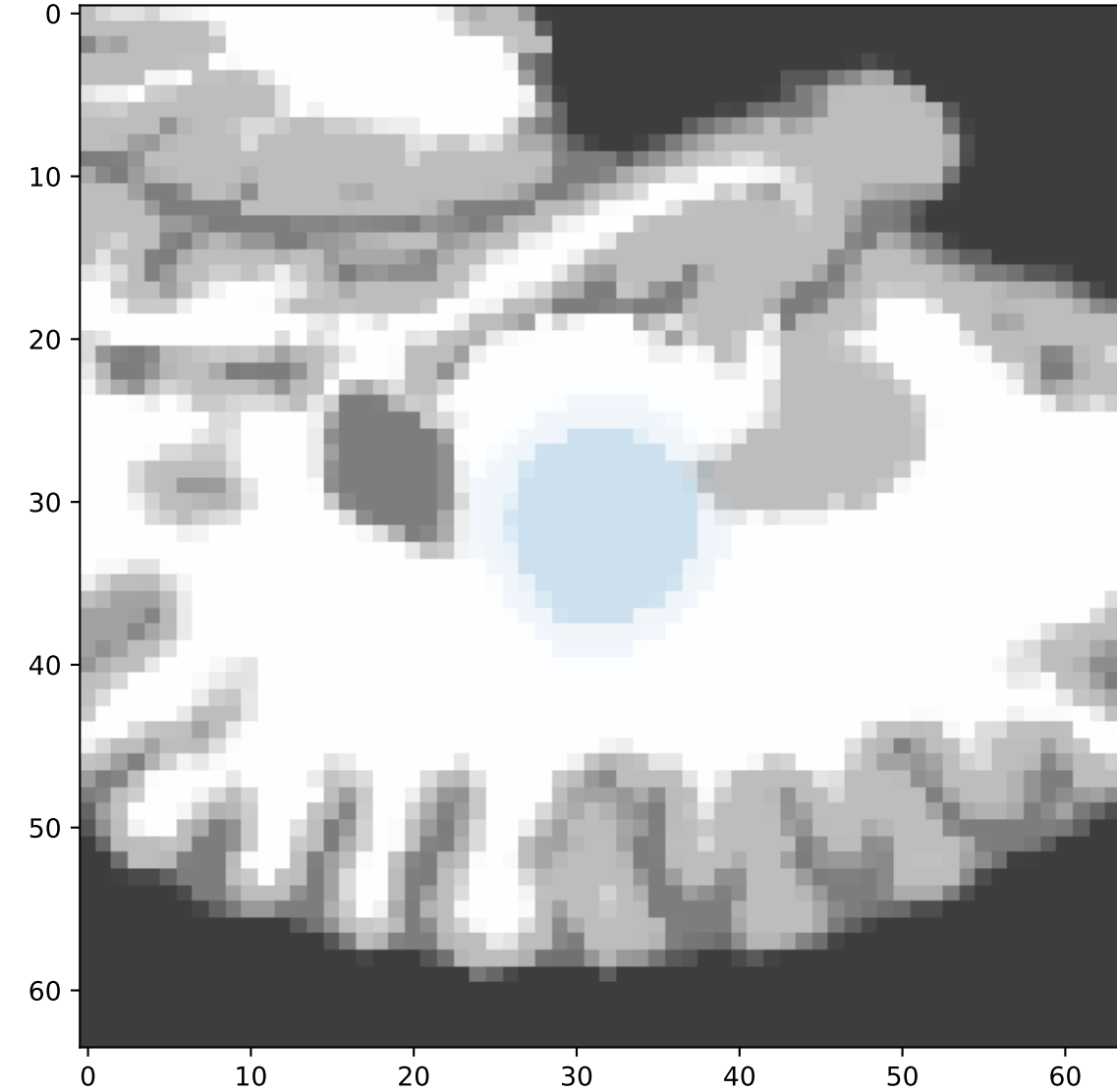
Step 100: Prediction
