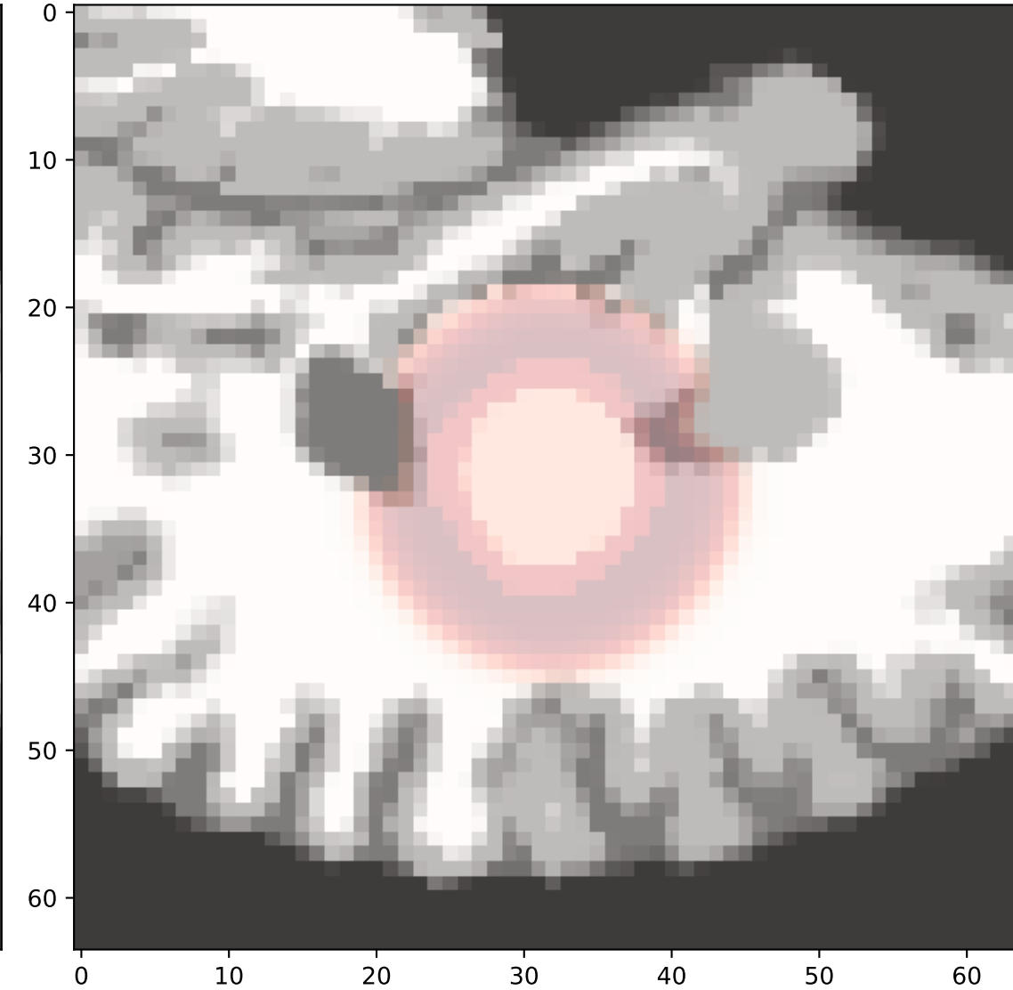
Step 100: Difference
