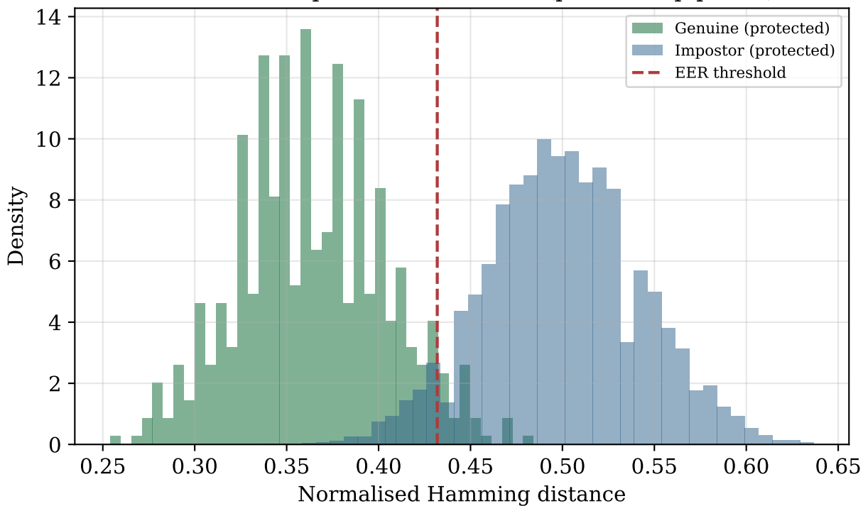
Genuine vs impostor distributions (protected pipeline)
