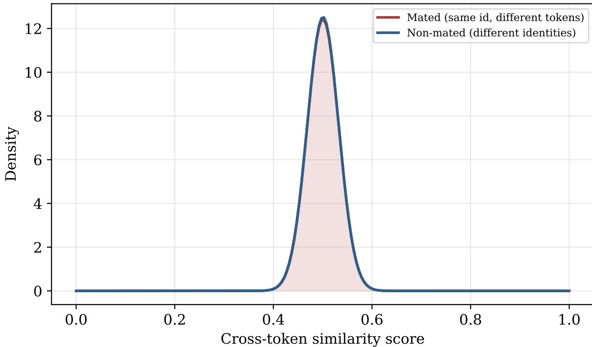
Unlinkability across tokens ( D_{\text{sys}} = 0.033 , 0 = fully unlinkable)
