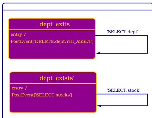
Figure 9: A Sample David HAREL-Statechart model of the temporal property expressed in fig. 4 : —" Whenever department YRI_ASSET was deleted (event 'DELETE.department.YRI_ASSET'); querying stock table shall not find again an inventory stock in any department named YRI_ASSET "—.
