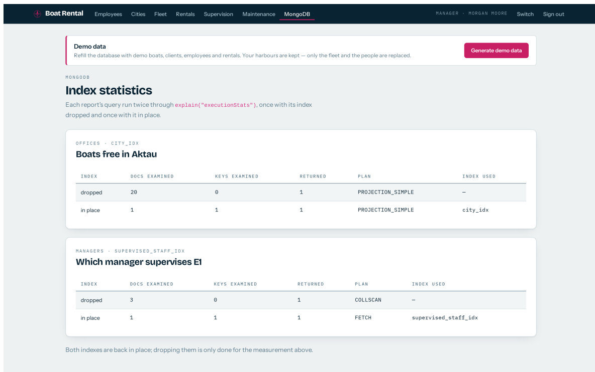
Figure 3: Execution statistics for both reports, each query run with its index dropped and then in place.
