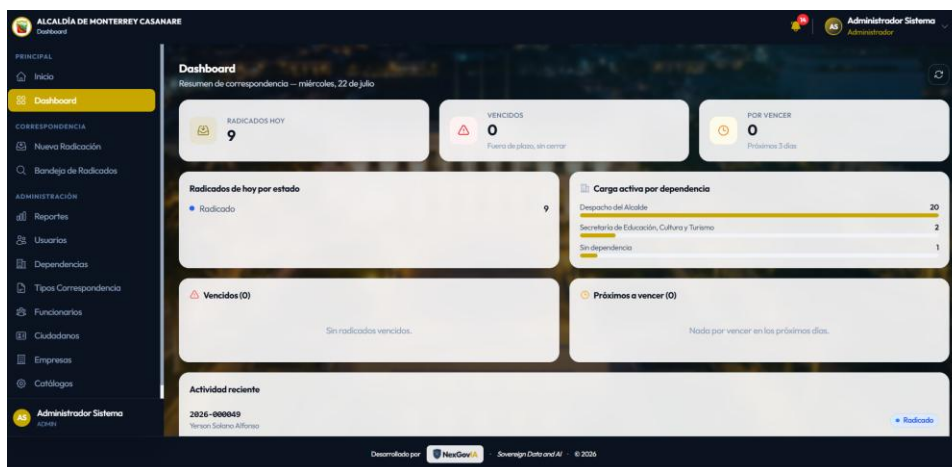
Figura 3. Dashboard
