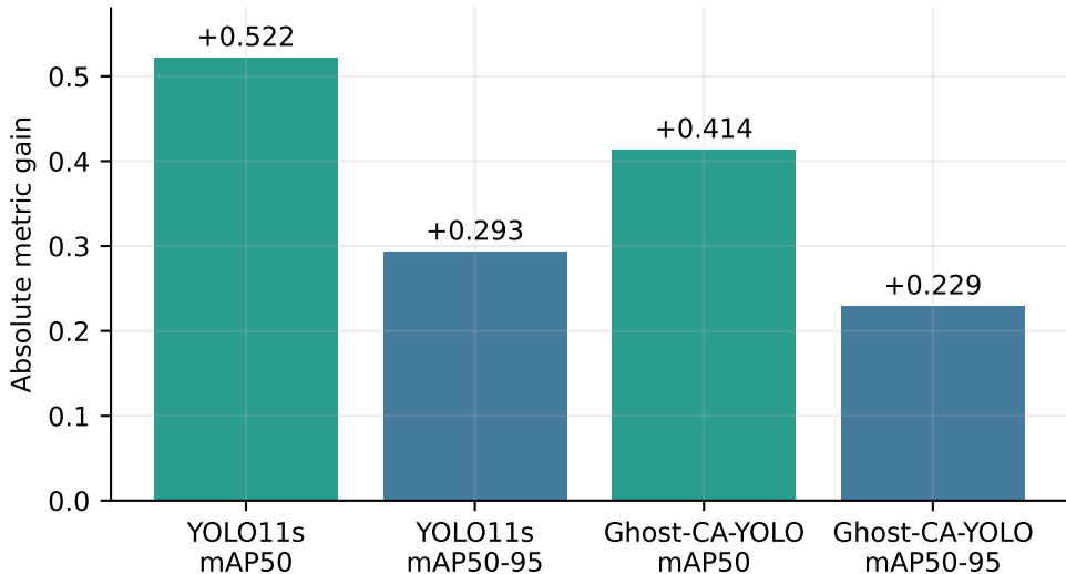
Kazakhstan fine-tuning gain over RDD-only transfer
