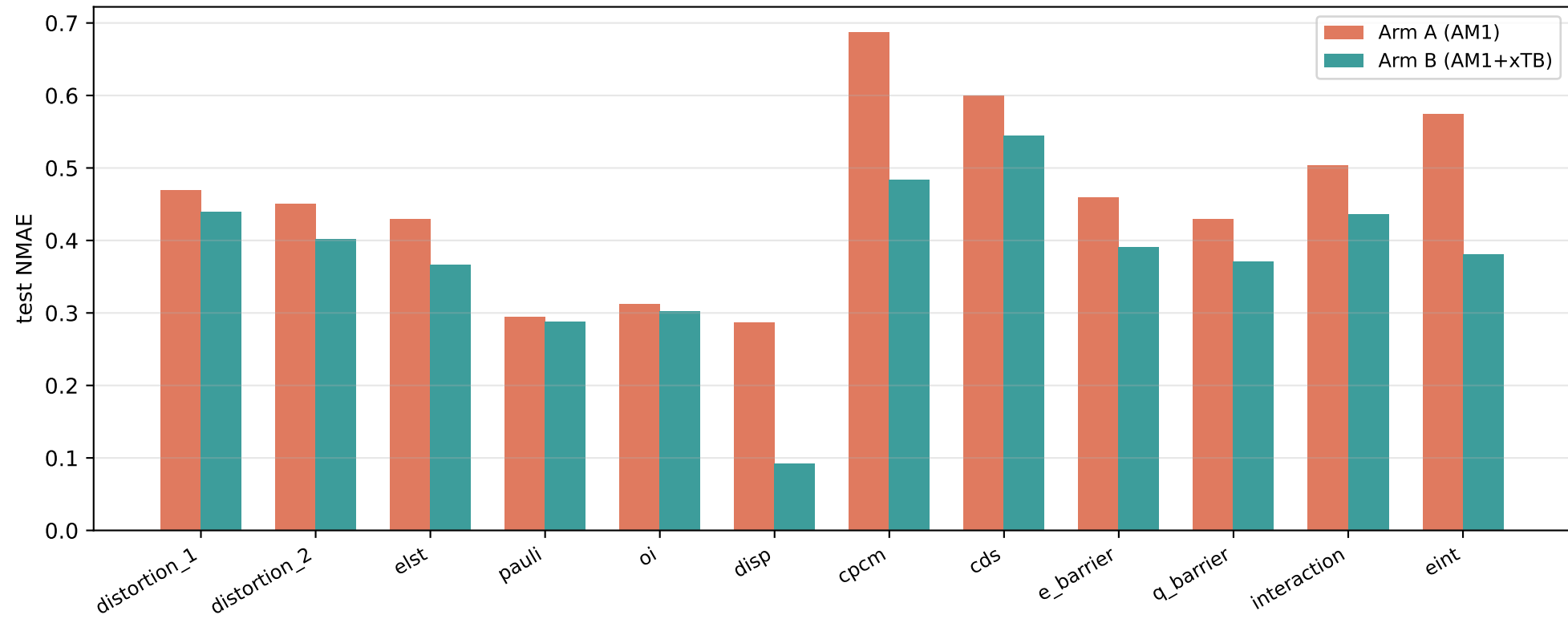
F1: NMAE per channel (5-seed mean, SVR) (model: SVR)
