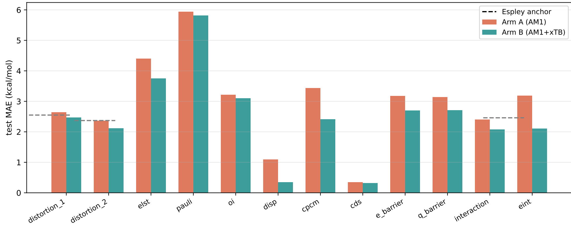
F2: MAE per channel (5-seed mean, SVR) (model: SVR)
