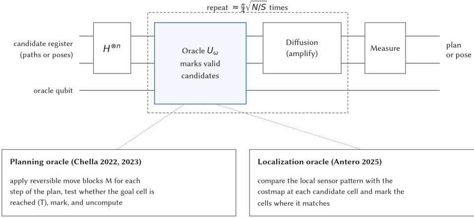
Fig. 5. Grover search as used for robot planning and localization. After a uniform superposition, the oracle marks goal-reaching action sequences [26, 27] or map cells whose stored pattern matches the current sensor view [4], and the diffusion step amplifies the marked states; about \frac{\pi}{4} \sqrt{N/S} repetitions are needed for N candidates and S solutions. Redrawn from the circuit descriptions in those studies.
